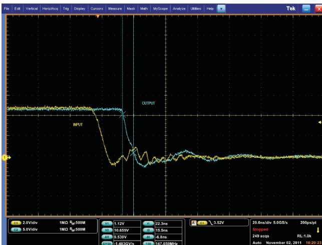
Figure 37. TurnOff Fall Time ( C_L = 1.8 \text{ nF} , V_{DD} = 12 \text{ V} )
