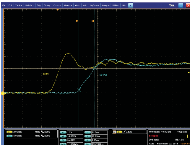
Figure 35. Turnon Rise Time ( C_L = 1.8 \text{ nF} , V_{DD} = 12 \text{ V} )
