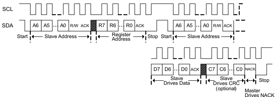
Figure 12. I²C Read Without Repeated Start
