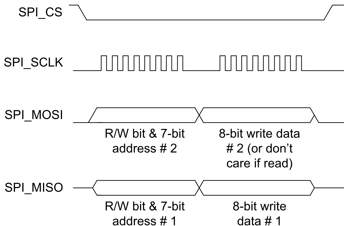
Figure 18. SPI Transaction #2 without CRC
