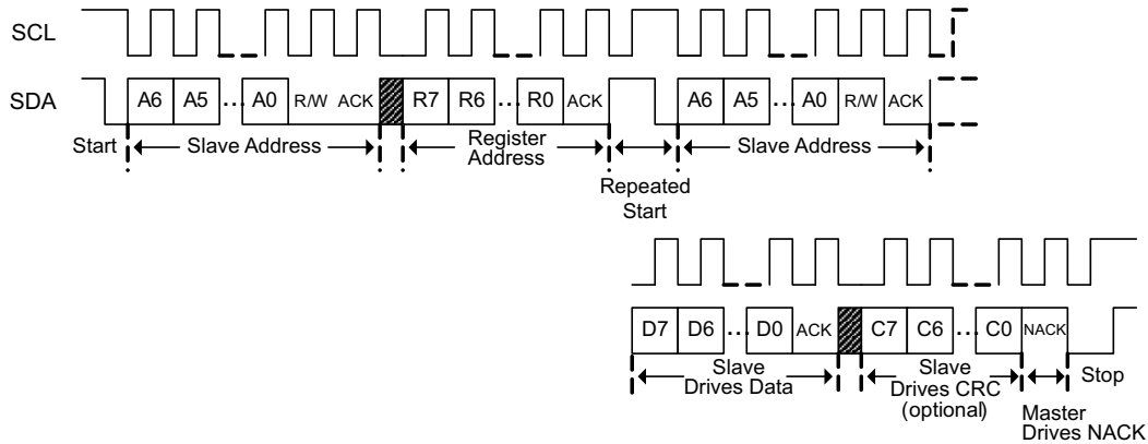
Figure 11. I²C Read with Repeated Start
