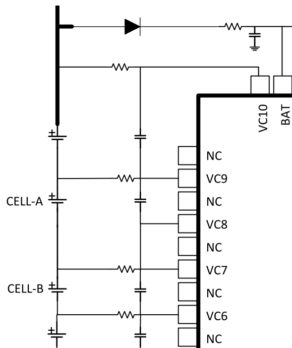
Figure 6. Terminating an unused cell input pin
