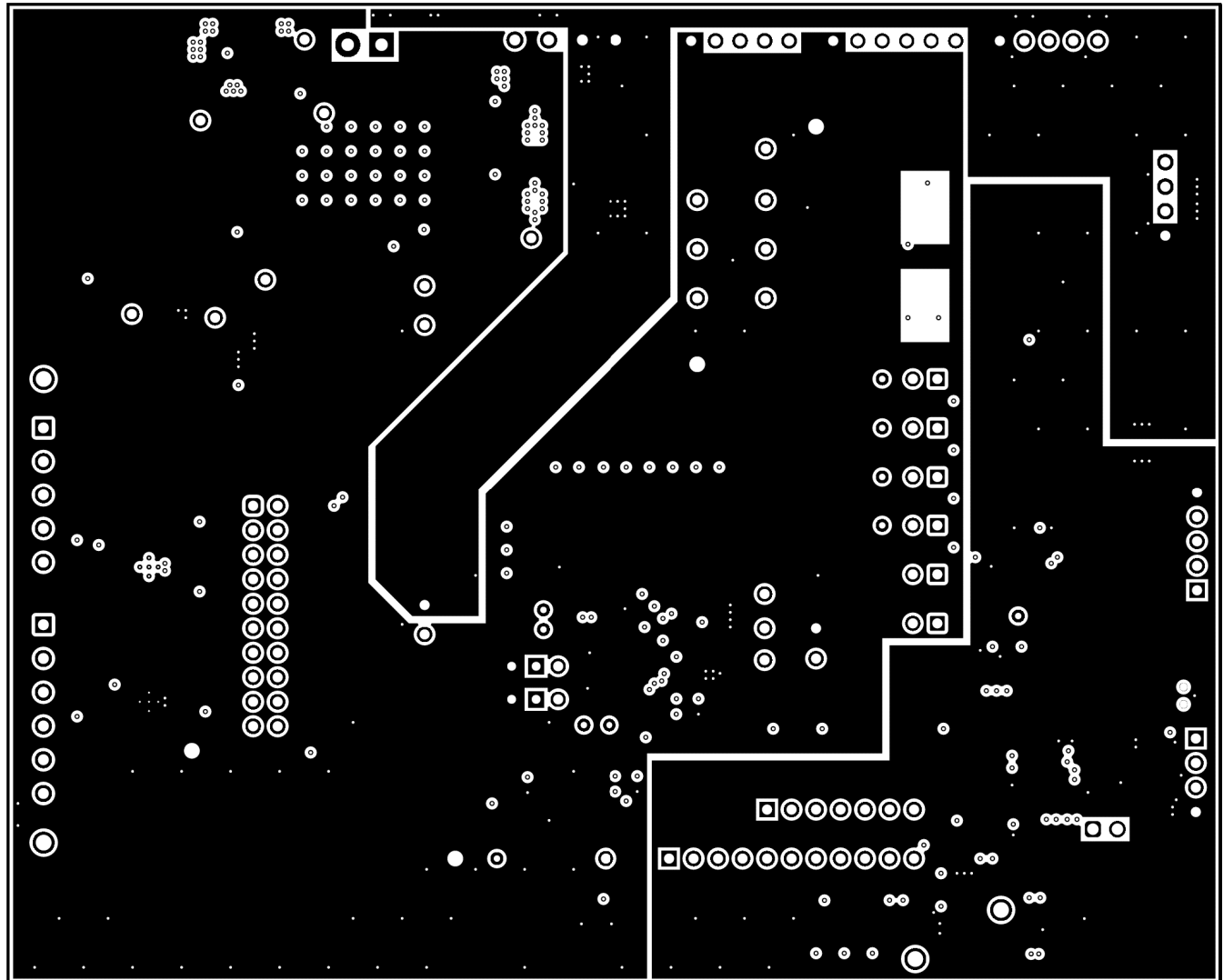
Figure 28. BQ76942 EVM Layer 2
