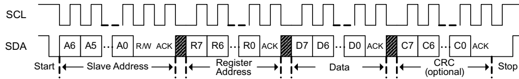
Figure 10. I²C Write
