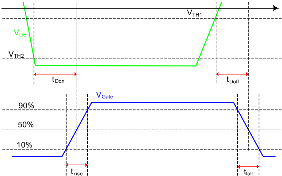
Fig. 15 - Timing Diagrams
