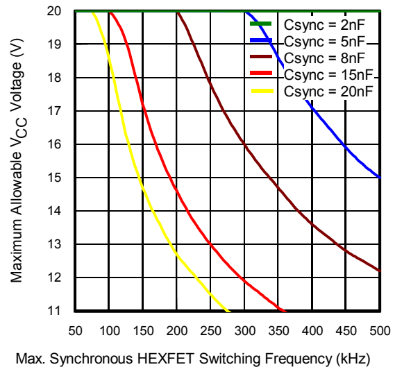
Fig 12. Max. V_{CC} Voltage vs. Synchronous Rectifier Switching Freq, T_J=125^\circ\text{C} , T_{IC} = 85^\circ\text{C} , external R_G=2\Omega , 1\Omega HEXFET Gate Resistance included
