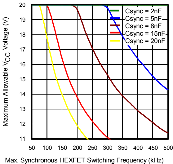
Fig 11. Max. V_{CC} Voltage vs. Synchronous Rectifier Switching Freq, T_J=125^\circ\text{C} , T_{IC} = 85^\circ\text{C} , external R_G=1\Omega , 1\Omega HEXFET Gate Resistance included
