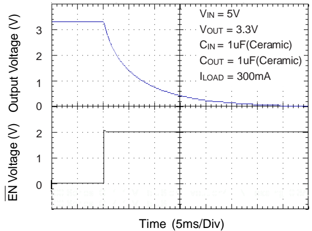
Enable Response
