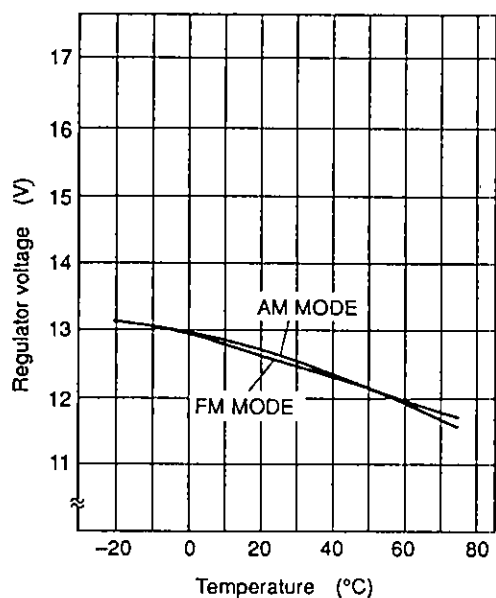
Temperature characteristics of regulator
