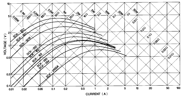
V-I CHARACTERISTIC CURVE FOR 10 φ SERIES
