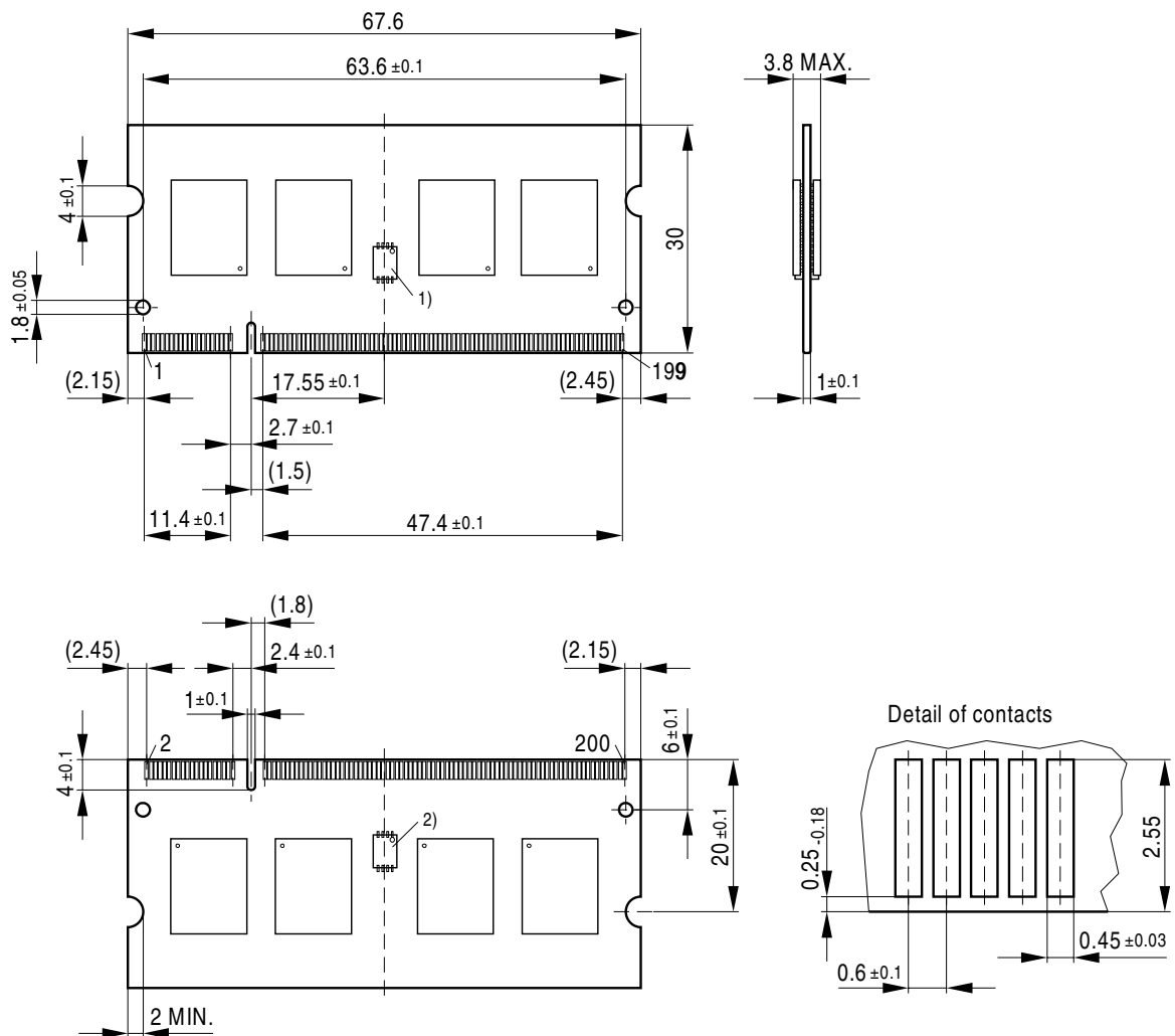
FIGURE 6 Package Outline Raw Card A L-DIM-200-31
