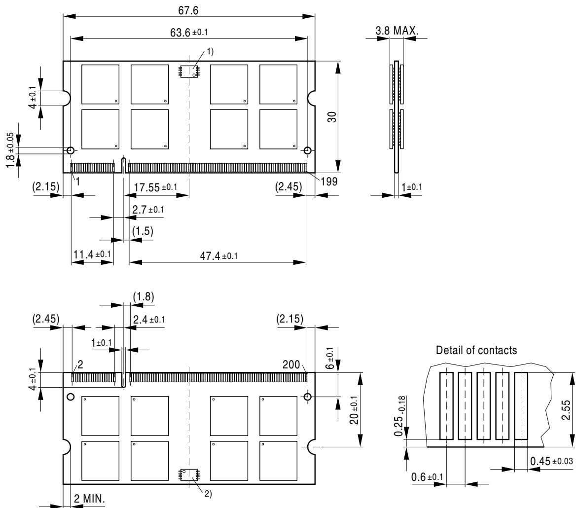
FIGURE 7 Package Outline Raw Card E L-DIM-200-36
