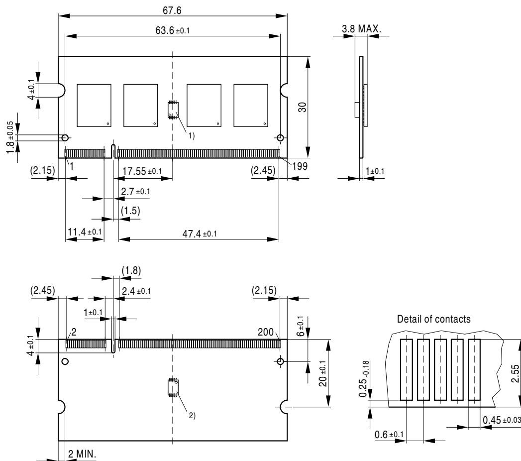
FIGURE 5 Package Outline Raw Card C L-DIM-200-30
