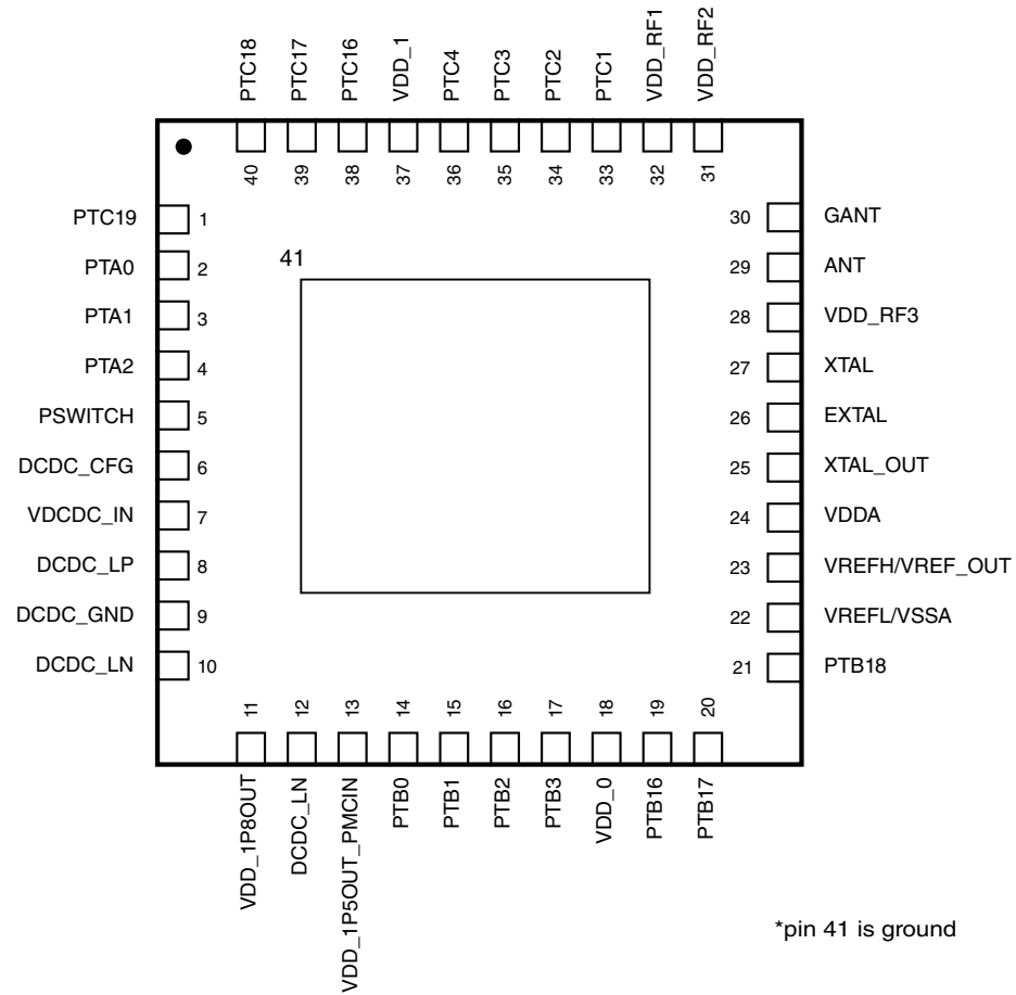
Figure 23. 40-pin "Wettable" HVQFN pinout diagram
