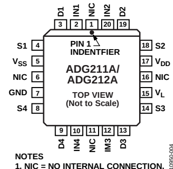
Figure 4. PLCC Pin Configuration
