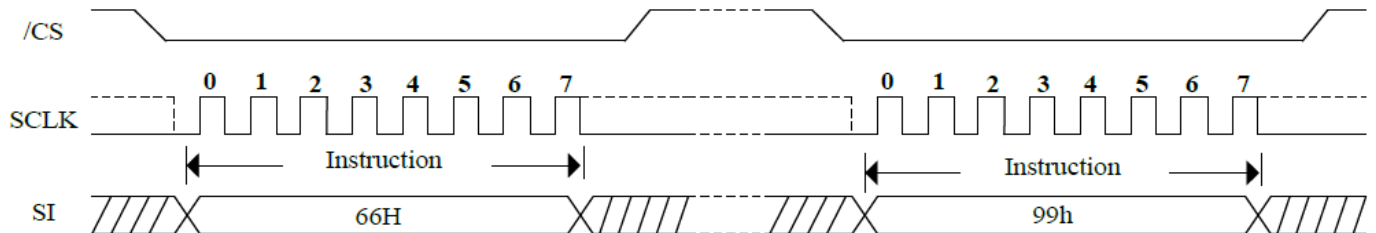
Figure 29. Enable Reset (66h) and Reset (99h) Command Sequence
