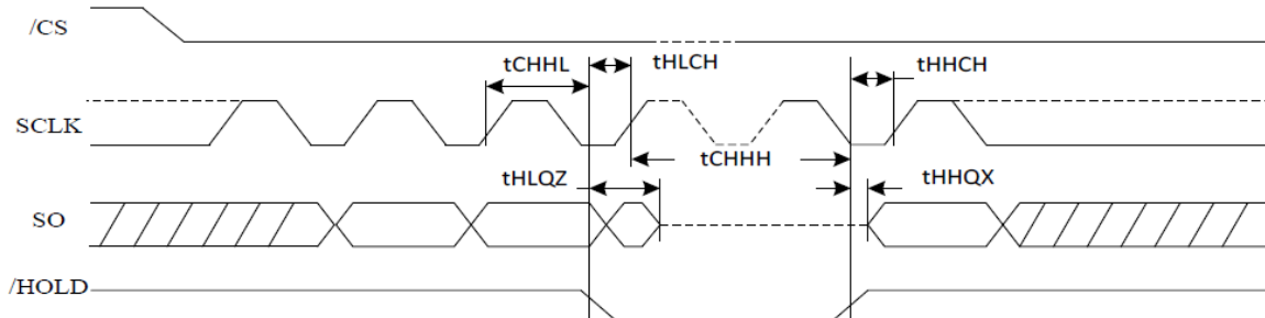
Figure 45. Hold Timing
