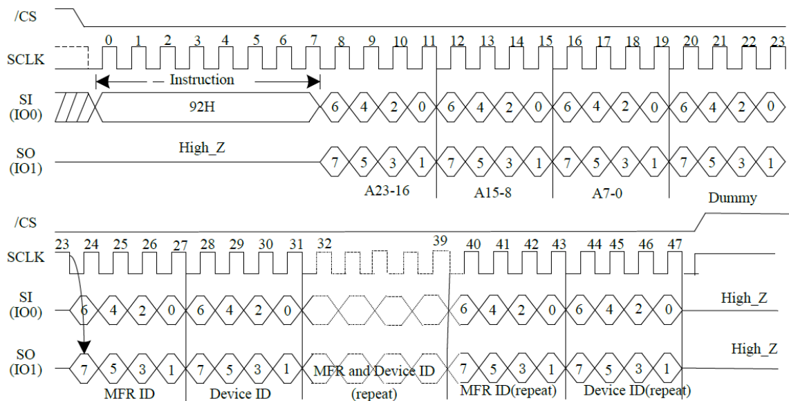
Figure 19. Dual I/O Read Manufacture ID/ Device ID Sequence Diagram
