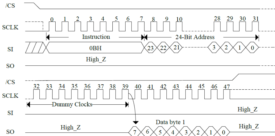
Figure 8. Fast Read Sequence Diagram
