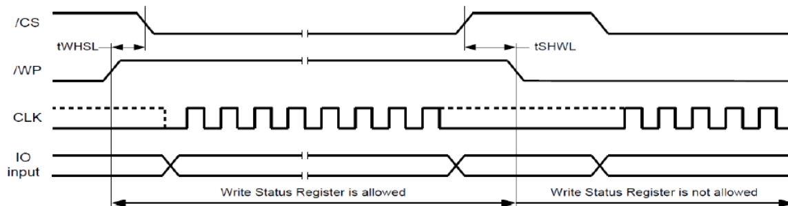
Figure 46. /WP Timing
