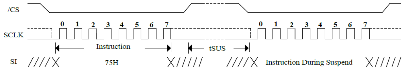
Figure 38. Erase/Program Suspend Command Sequence
