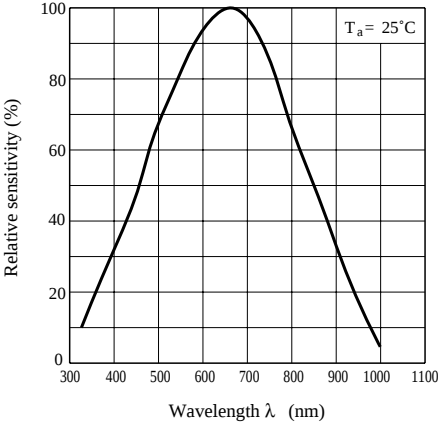
Fig. 9 Spectral Sensitivity
