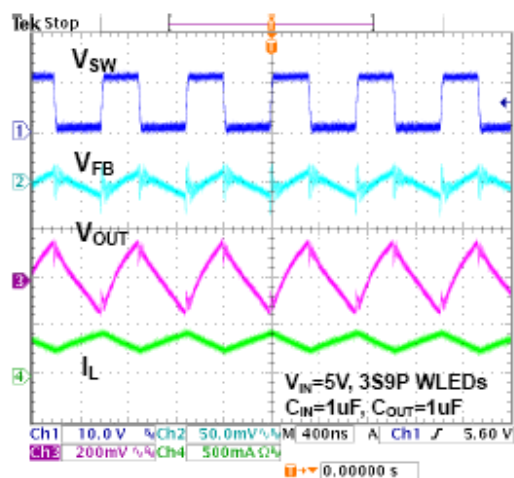
Figure 4. Switch waveforms
