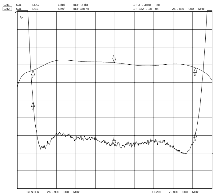
Passband Amplitude & Group Delay (1 dB/div & 5 nsec/div)
