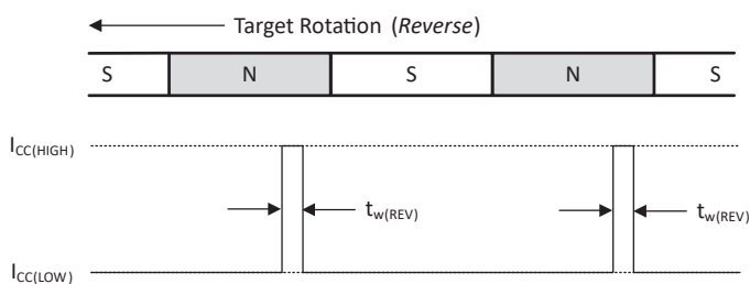
Figure 8: Output Protocol (-Fxxxxxx), No High Speed Mode, Reverse Rotation
