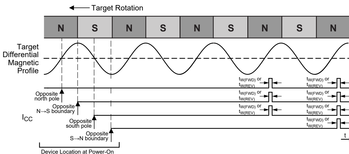
Figure 11: Startup Position Effect on First Device Output Switching (-xxxxxOxx variant)
