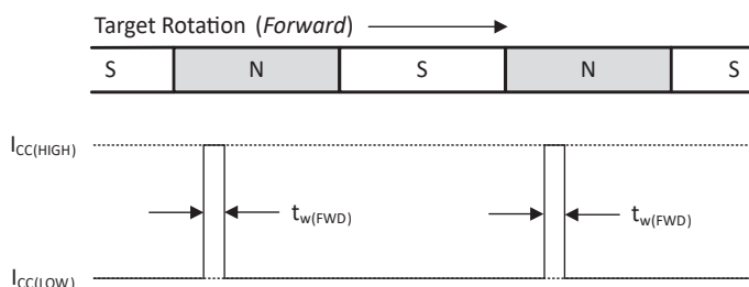
Figure 7: Output Protocol (-Fxxxxxx), No High Speed Mode, Forward Rotation
