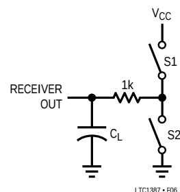
Figure 6. Receiver Output Enable/Disable Timing Test Load
