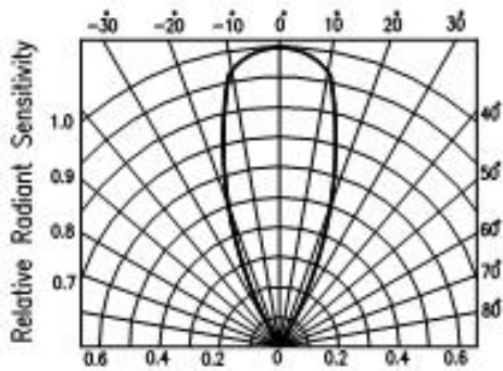
Fig. 7 Relative Radiant Sensitivity vs. Angular Displacement
