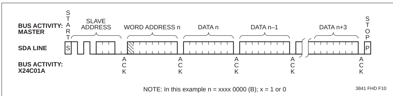
Figure 6. Page Write
