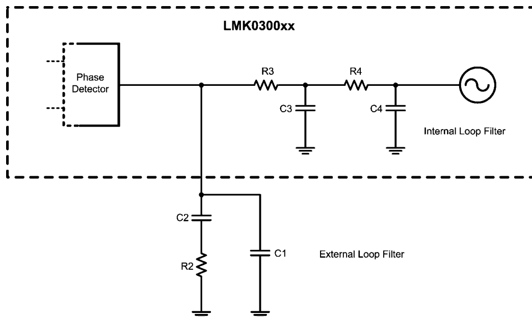
FIGURE 4. Loop Filter
