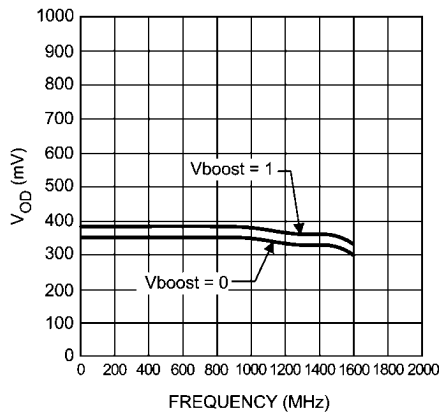
LVDS Differential Output Voltage ( V_{OD} )
