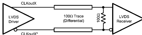
FIGURE 6. Differential LVDS Operation, DC Coupling
