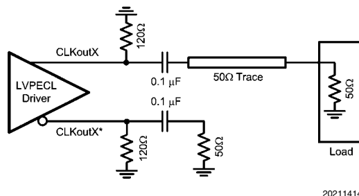
FIGURE 13. Single-Ended LVPECL Operation, AC Coupling
