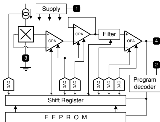
Figure 1-1 Functional Diagram
