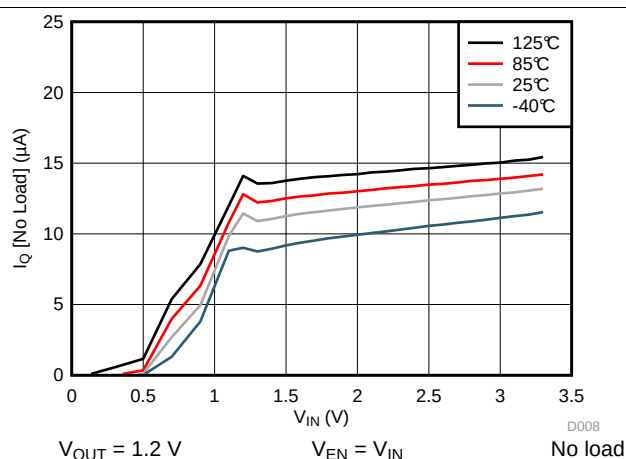
Figure 8. I_Q vs V_{IN}
