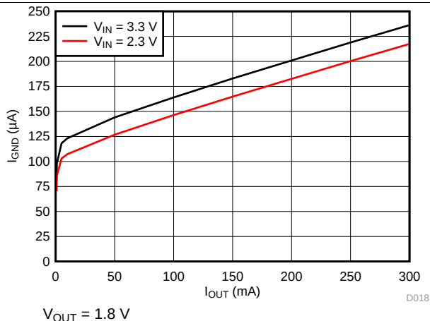
Figure 18. I_{GND} vs I_{OUT}
