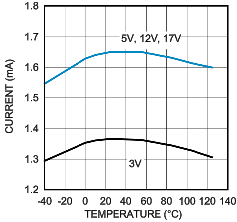
VIN Pin Current (Enabled)
