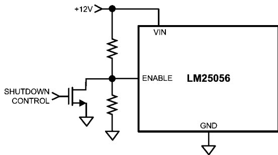
FIGURE 1. ENABLE Control
