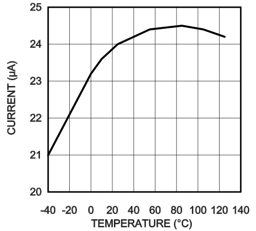
VS- Pin Input Bias Current (Enabled)
