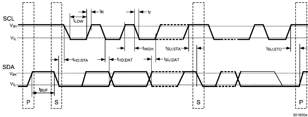
FIGURE 5. SMBus Timing Diagram
