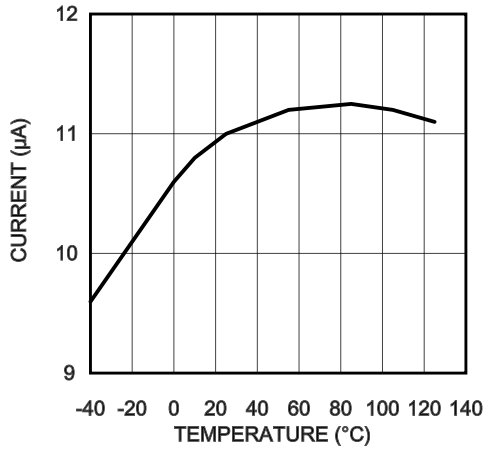
VS+ Pin Input Bias Current (Enabled)
