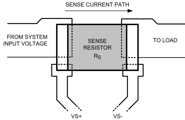
FIGURE 3. Sense Resistor Connections
