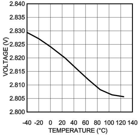
VREF Voltage
