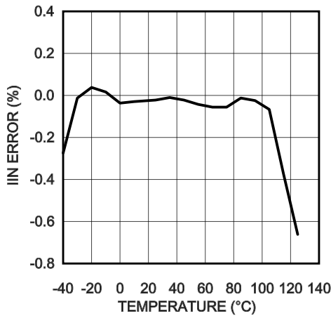
IIN Error, GAIN=0, V SENSE =25mV
