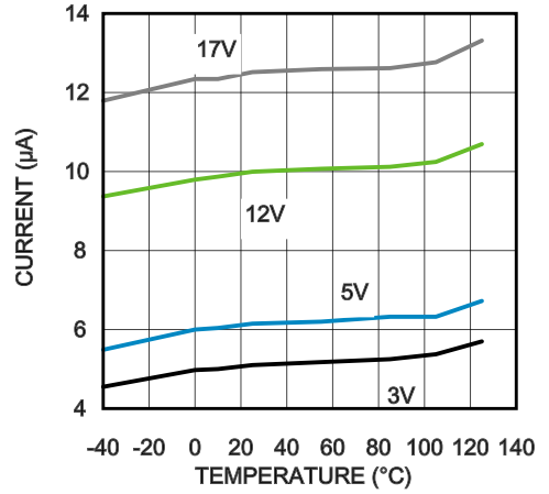
VIN Pin Current (Disabled)
