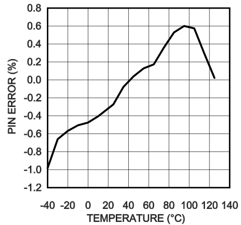
PIN Error, GAIN=0, VIN=12V, V SENSE =25mV
