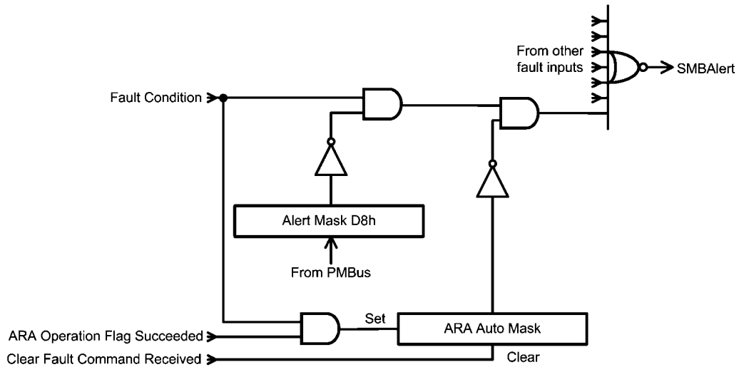
FIGURE 6. Typical Flow Schematic for \overline{\text{SMBA}} Fault
