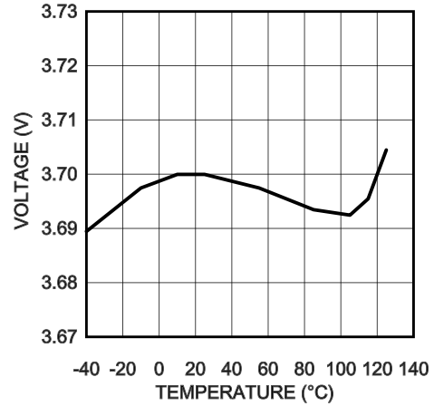
VDD Voltage
