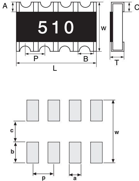
4-Resistor Device
