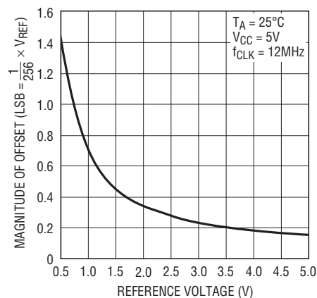
Offset vs Reference Voltage
