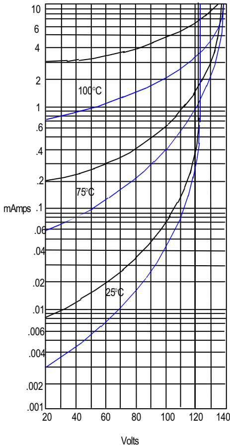
Figure 4 Typical Reverse Characteristics
