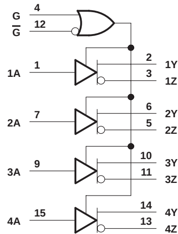
logic diagram (positive logic)
