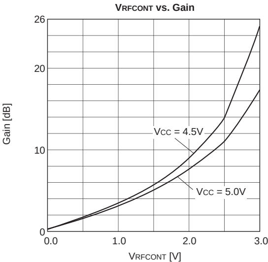
CL mode RFGCA gain control supply voltage characteristics
