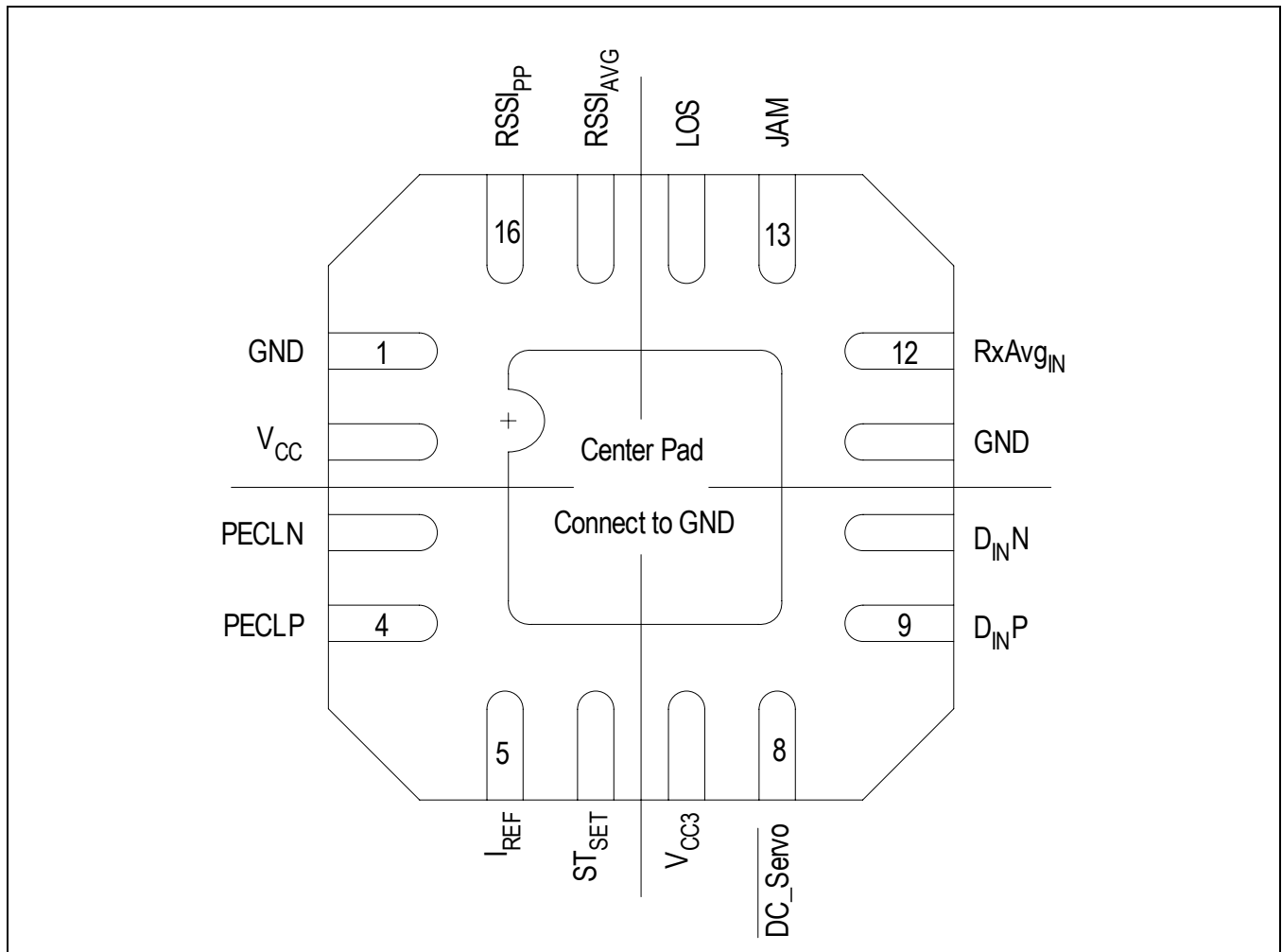
Figure 2-1. M02040-15 Pinout
