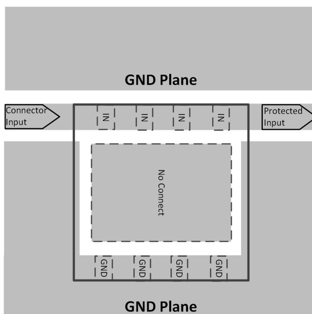
Figure 3. TVS2701 Layout
