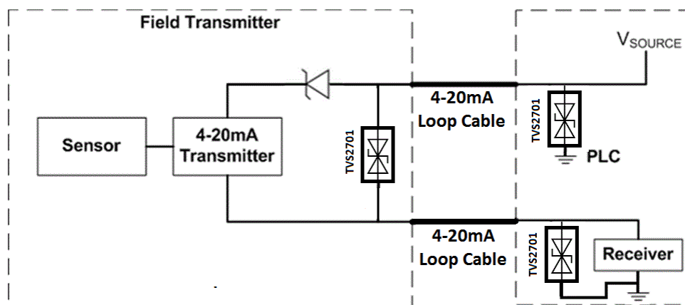
Figure 1. TVS2701 Application Example
