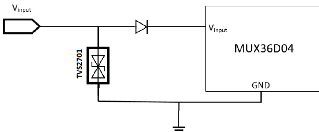
Figure 2. TVS2701 Application Schematic
