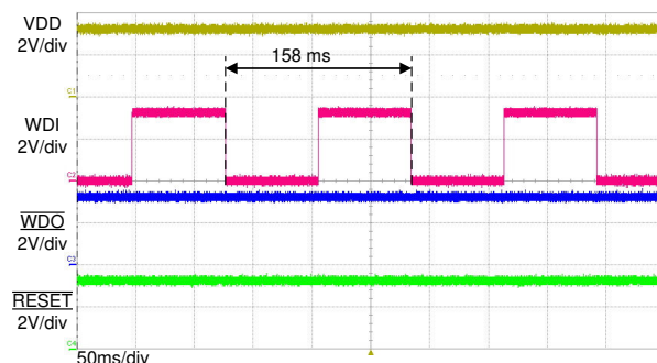
图 8-14. Typical WDI Signal
