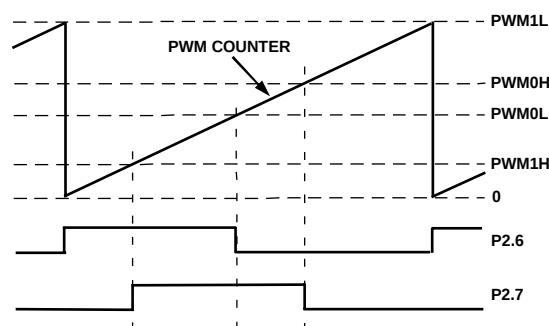
Figure 49. PWM Mode 2
