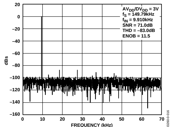
Figure 18. Dynamic Performance at V_{DD} = 3\text{ V}
