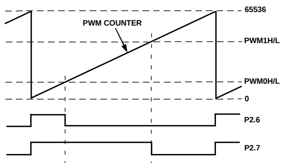
Figure 50. PWM Mode 3
