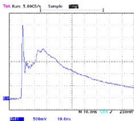
Pulse Waveform
