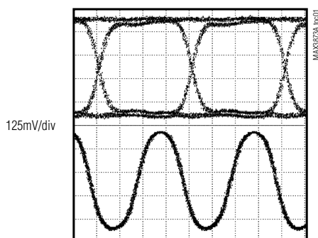
RECOVERED CLOCK AND DATA (2.488Gbps, 2^{23} - 1 PATTERN, V_{IN} = 50\text{mVp-p} )
