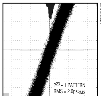
RECOVERED CLOCK JITTER (2.488Gbps)
