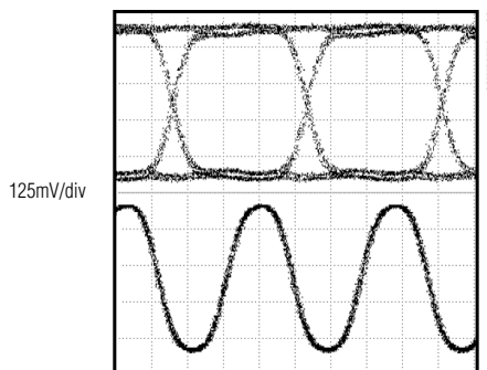
RECOVERED CLOCK AND DATA (2.67Gbps, 2^{23} - 1 PATTERN, V_{IN} = 50\text{mVp-p} )
