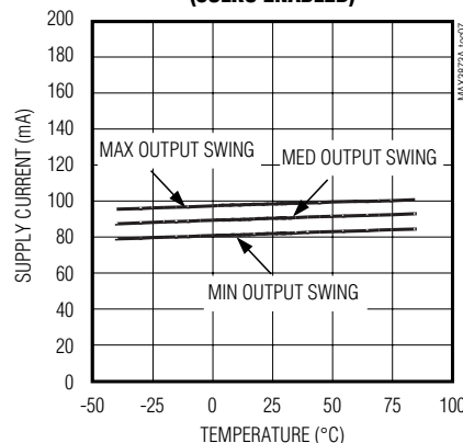
SUPPLY CURRENT vs. TEMPERATURE (SCLKO ENABLED)
