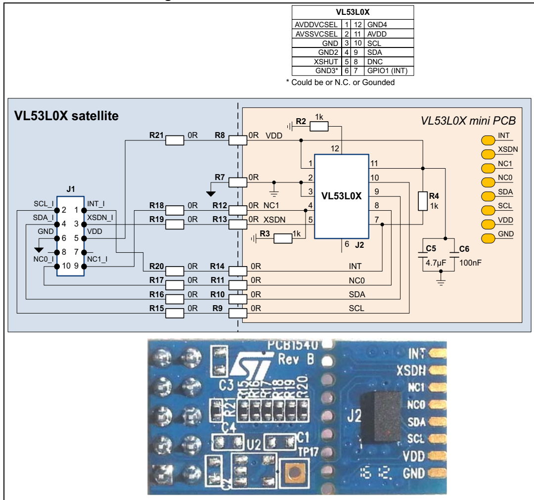
Figure 7. VL53L0X satellite schematic
