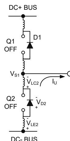
Figure 13 V_S negative
