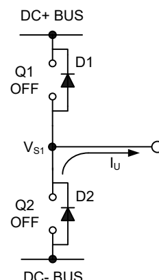
Figure 8 D2 conducting
