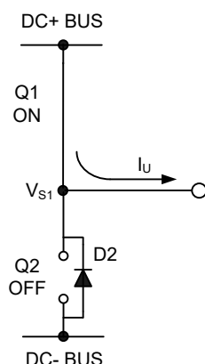
Figure 7 Q1 conducting
