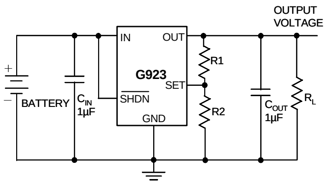
Figure 2. Adjustable Output Using External Feedback Resistors
