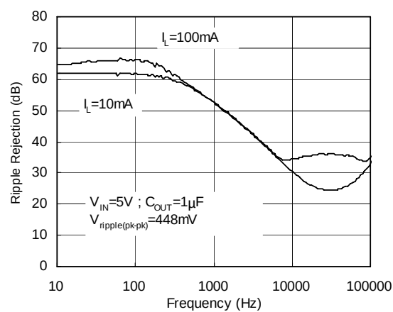
Ripple Rejection
