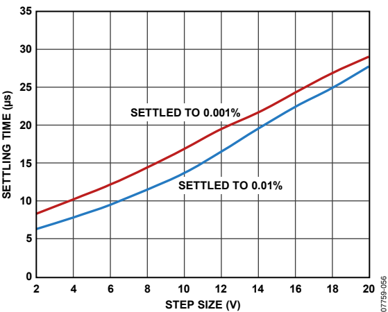
Figure 56. Settling Time vs. Step Size, V_S = \pm 15 V, Dual Supply
