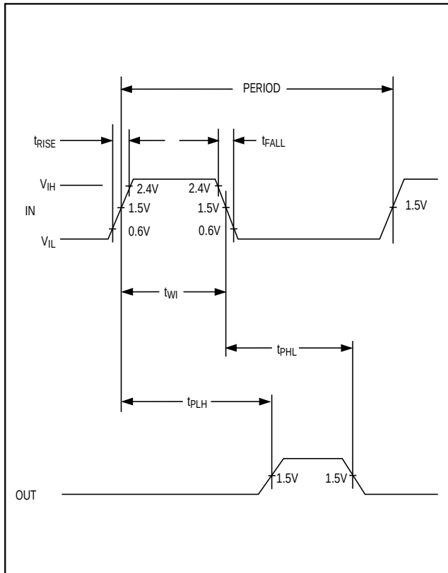
Figure 1. Timing Diagram
