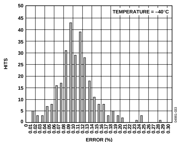
Figure 36. Gain Accuracy, SOIC, Temperature = -40^{\circ}\text{C}
