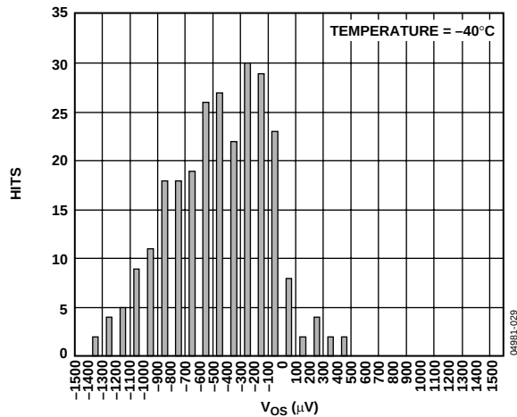
Figure 30. V_{OS} Distribution, SOIC, Temperature = -40^{\circ}\text{C}
