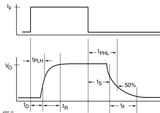
Figure 1. Switching Waveform
