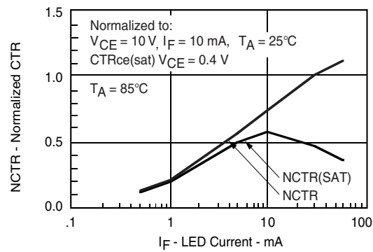
Figure 7. Normalized Non-saturated and saturated CTR vs. LED Current
