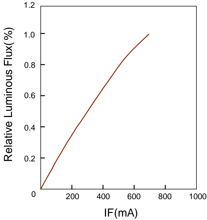
Fig.3 Forward current vs. Luminous Flux
