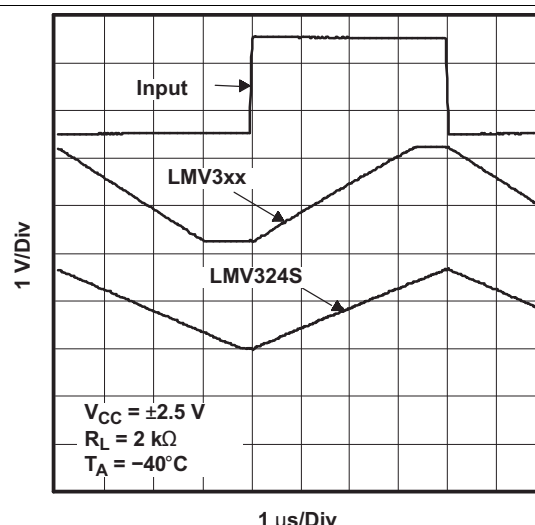
Figure 24. Noninverting Large-Signal Pulse Response
