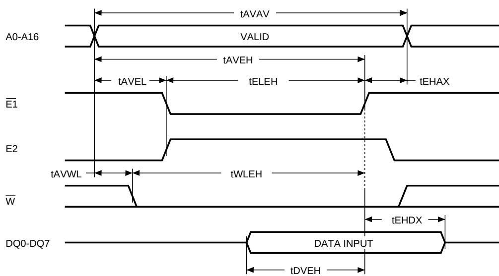
Figure 12. Chip Enable Controlled, Write AC Waveforms
