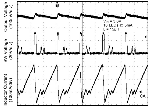
TIME (1µs/div)
