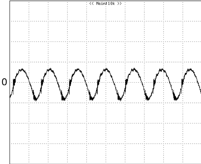
Figure 11: Input Terminal Ripple Current, i_c , at full rated output current and nominal input voltage with 12\mu\text{H} source impedance and 33\mu\text{F} electrolytic capacitor (500 mA/div, 2 \mu\text{s} /div)
