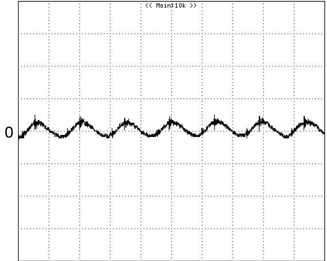
Figure 12: Input reflected ripple current, i_s , through a 12\mu\text{H} source inductor at nominal input voltage and rated load current (20 mA/div, 2 \mu\text{s} /div)
