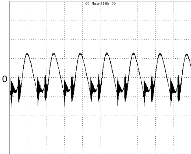
Figure 14: Output voltage ripple at nominal input voltage and rated load current ( I_o=25A ) (10 mV/div, 2 \mu s/div)
