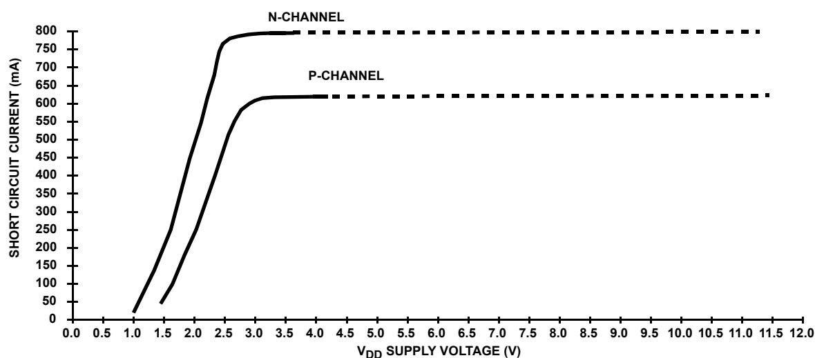
FIGURE 7. TYPICAL CHARACTERISTIC OF THE P AND N OUTPUT DRIVER SHORT CIRCUIT CURRENT vs SUPPLY VOLTAGE, T_{AMBIENT} = 25^{\circ}C
