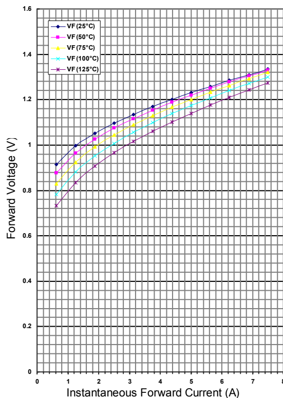
Typical Forward Characteristic
