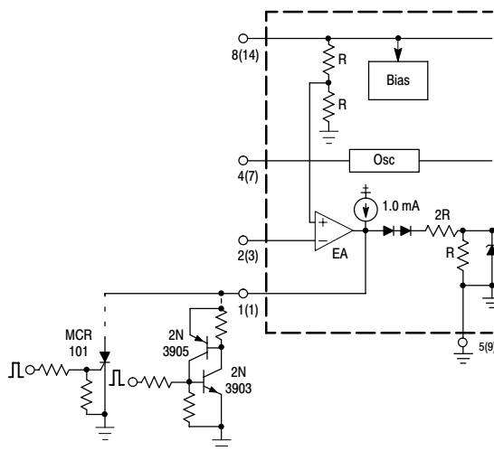
Figure 31. Latched Shutdown
