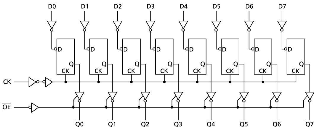
TC74HC574A
