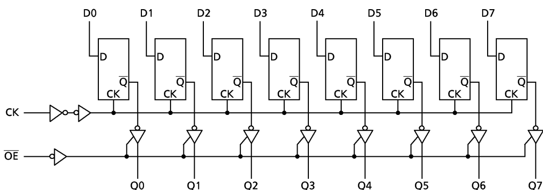
TC74HC574A
