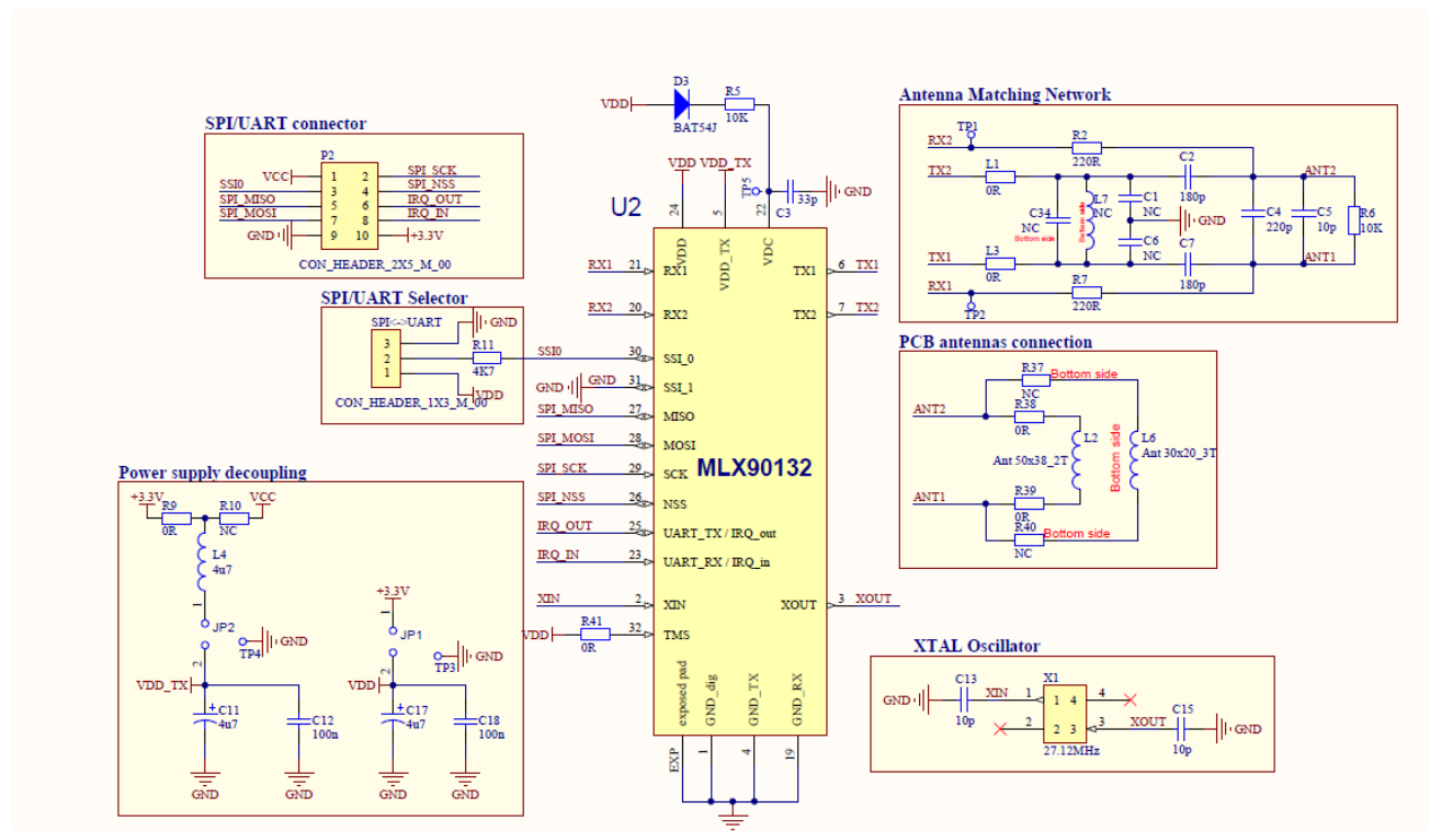
Figure 2: Schematics MLX90132
