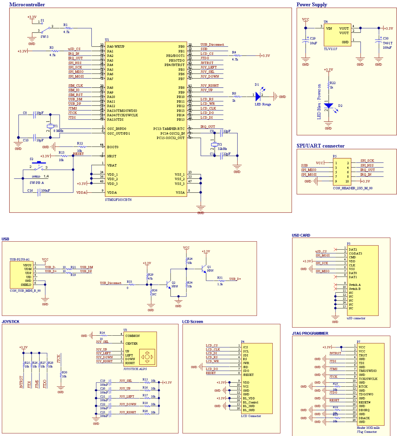
Figure 3: Schematics Microcontroller & Peripherals
