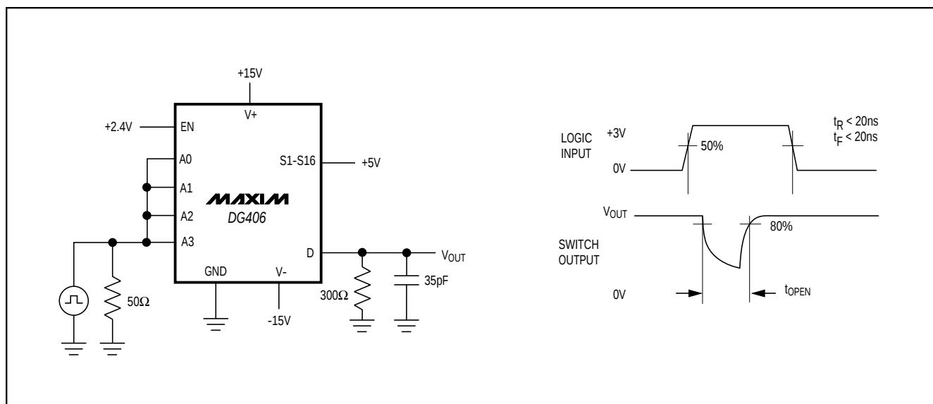
Figure 4. Break-Before-Make Interval
